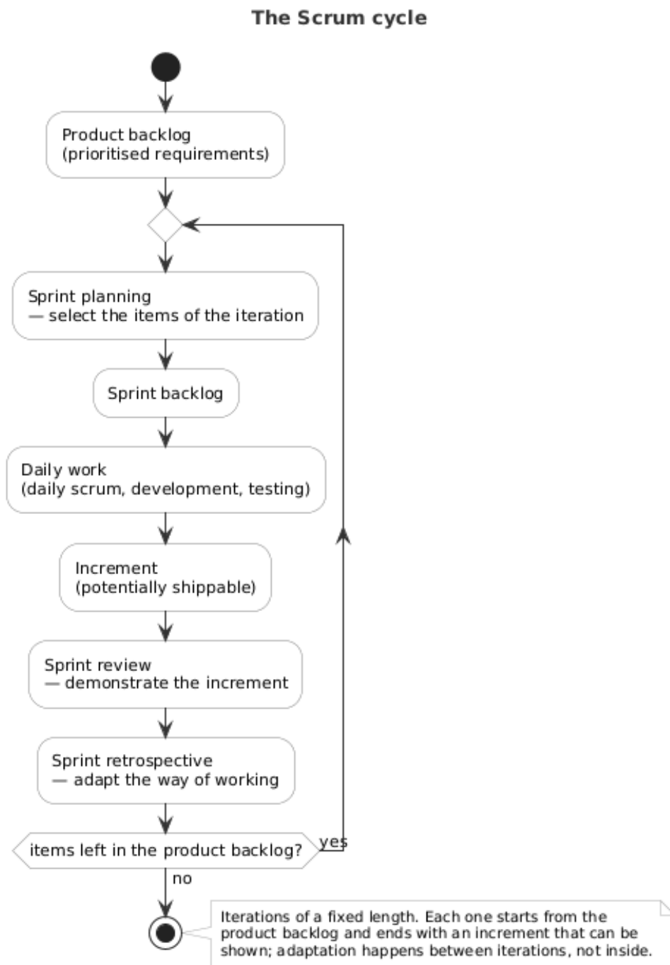
Figure 1.15: The Scrum cycle
